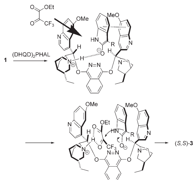
Scheme 2. Conformation of the (DHQD) 2 PHAL catalyst and proposed approximate structure of the substrate-catalyst complex for the S,S -selective formation of adducts 3 in the aldol-type condensation of oxindoles 1 with 2 .
